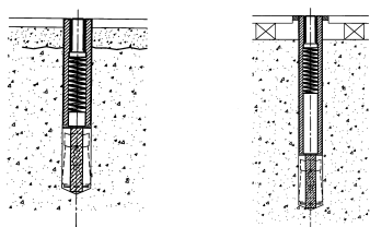
Standard Floor Plug Semi-Sprung Floor Plug
